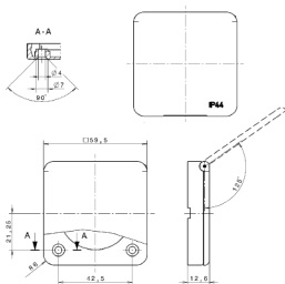
Drawing 1 MB 422 Dim. in mm
