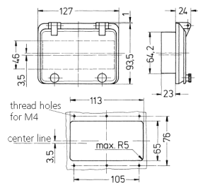
Drawing 6 MB 17 Dim. in mm
