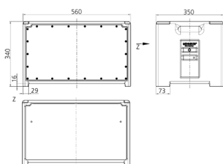
Drawing 5 MB 70 Dim. in mm
