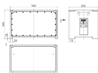
Drawing 5 MB 70 Dim. in mm
