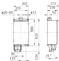
Drawing 1 MB 387 Dim. in mm
