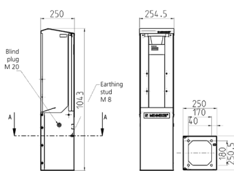
Drawing 1 MB 517 Dim. in mm
