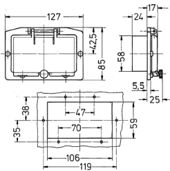
Drawing 6 MB 2 Dim. in mm
