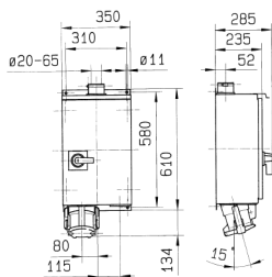
Drawing 1 MB 386 Dim. in mm
