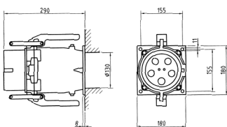
Drawing 2 MB 199/1 Dim. in mm
