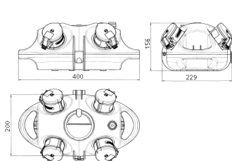
Drawing 1 MB 441
