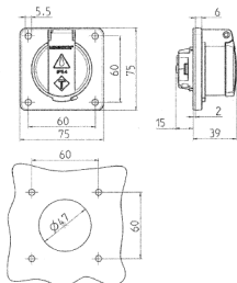
Drawing 1 MB 592 Dim. in mm
