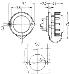
Drawing 1 MB 301 Dim. in mm
