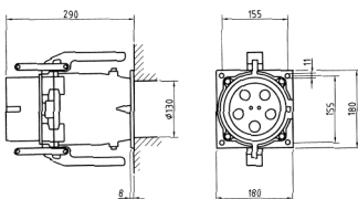
Drawing 2 MB 199/1 Dim. in mm
