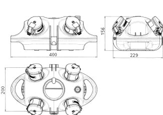
Drawing 1 MB 441
