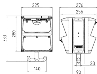
Drawing 1 MB 630
