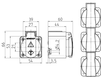
Drawing 1 MB 27/30 Dim. in mm
