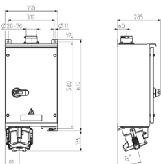
Drawing 1 MB 728 Dim. in mm
