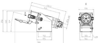
Drawing 1 MB 385 Dim. in mm
